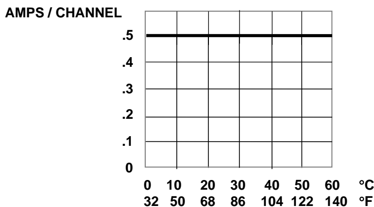
Derating Chart
