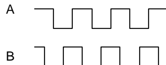
Figure 5.4 - Count DOWN (4x)
