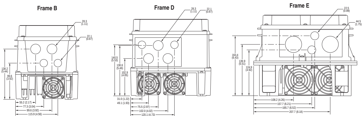
Figure 3 - IP 66 (NEMA/UL Type 4X/12) Bottom View Dimensions, mm (in.)
