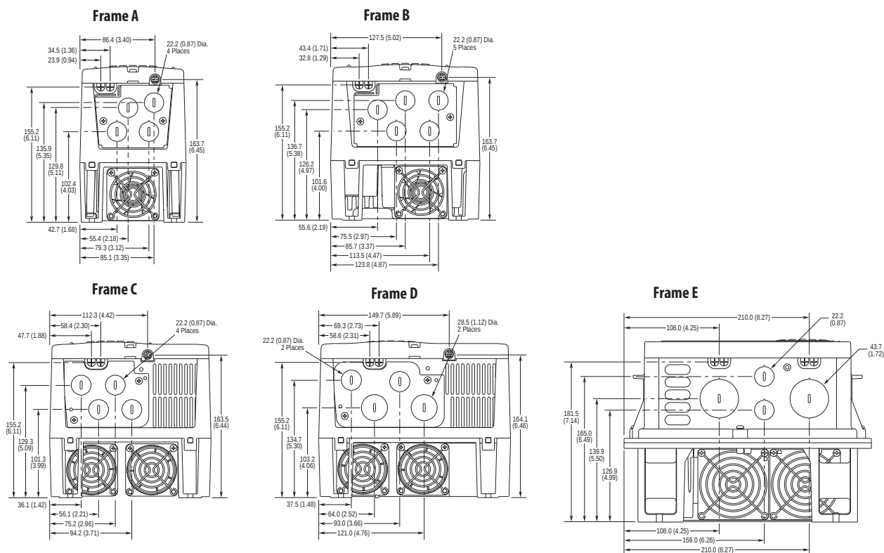
Figure 3 - IP 66 (NEMA/UL Type 4X/12) Bottom View Dimensions, mm (in.)
